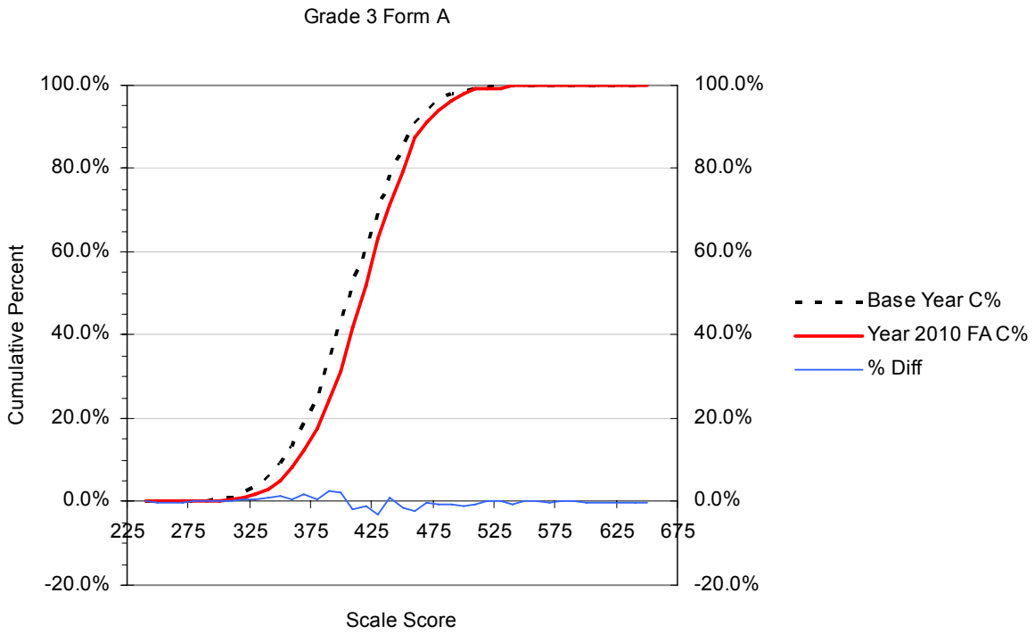
Figure B.3 Cumulative Distribution Functions (CDFs) for the Year 2006 vs. Year 2010 Scale Scores with the Percent Differences between CDFs: Grade 3 Form A
