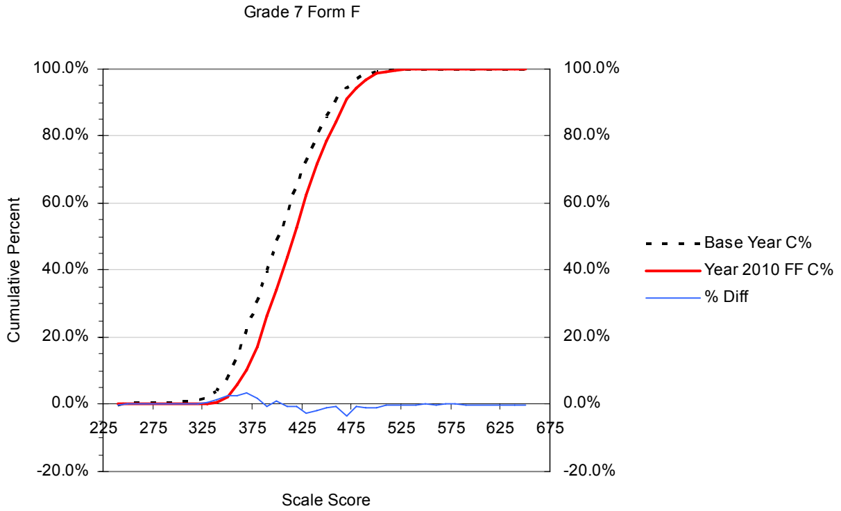
Figure B.34 Cumulative Distribution Functions (CDFs) for the Year 2006 vs. Year 2010 Scale Scores with the Percent Differences between CDFs: Grade 7 Form F
