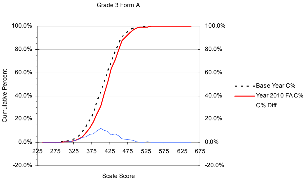
Figure B.4 Cumulative Distribution Functions (CDFs) for the Year 2006 vs. Year 2010 Scale Scores with the Cumulative Percent Differences between CDFs: Grade 3 Form A
