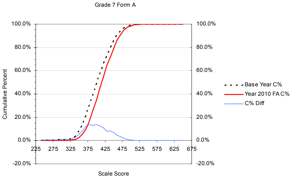
Figure B.32 Cumulative Distribution Functions (CDFs) for the Year 2006 vs. Year 2010 Scale Scores with the Cumulative Percent Differences between CDFs: Grade 7 Form A
