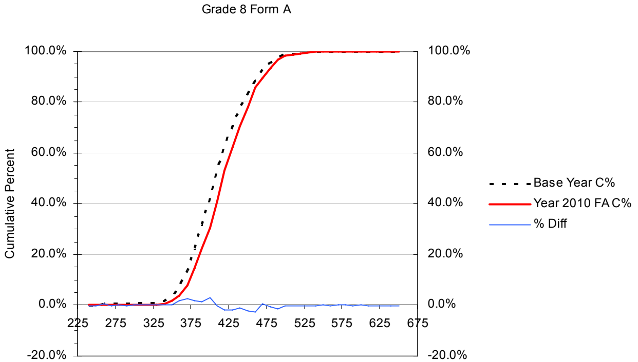
Figure B.38 Cumulative Distribution Functions (CDFs) for the Year 2006 vs. Year 2010 Scale Scores with the Percent Differences between CDFs: Grade 8 Form A
