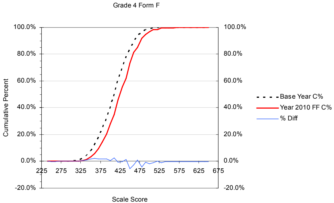
Figure B.13 Cumulative Distribution Functions (CDFs) for the Year 2006 vs. Year 2010 Scale Scores with the Percent Differences between CDFs: Grade 4 Form F
