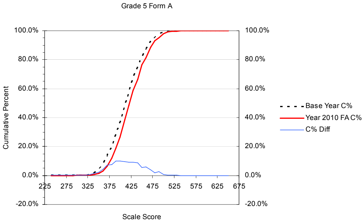
Figure B.17 Cumulative Distribution Functions (CDFs) for the Year 2006 vs. Year 2010 Scale Scores with the Percent Differences between CDFs: Grade 5 Form A
