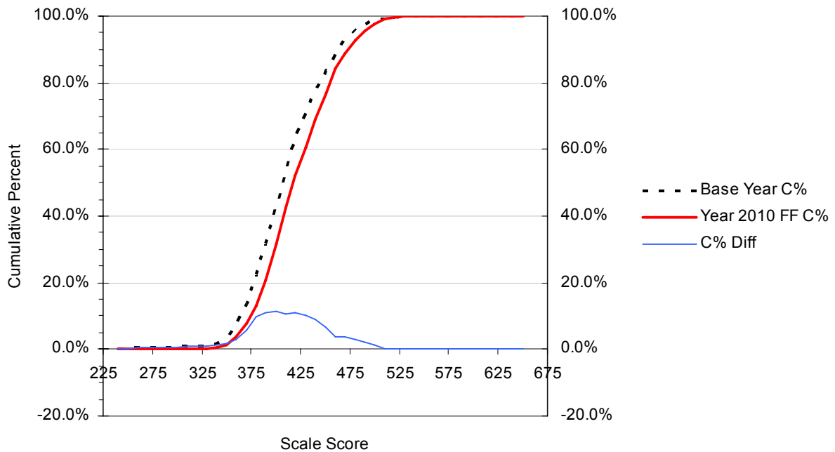
Figure B.42 Cumulative Distribution Functions (CDFs) for the Year 2006 vs. Year 2010 Scale Scores with the Cumulative Percent Differences between CDFs: Grade 8 Form F
