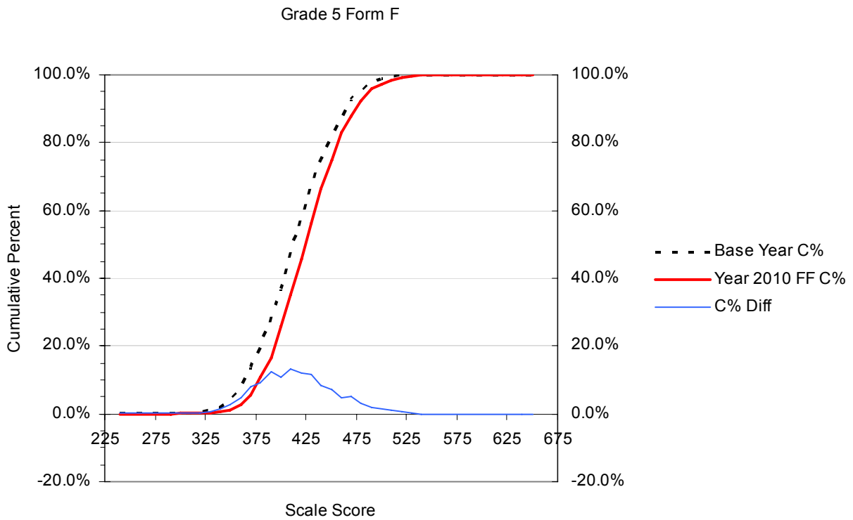
Figure B.21 Cumulative Distribution Functions (CDFs) for the Year 2006 vs. Year 2010 Scale Scores with the Cumulative Percent Differences between CDFs: Grade 5 Form F
