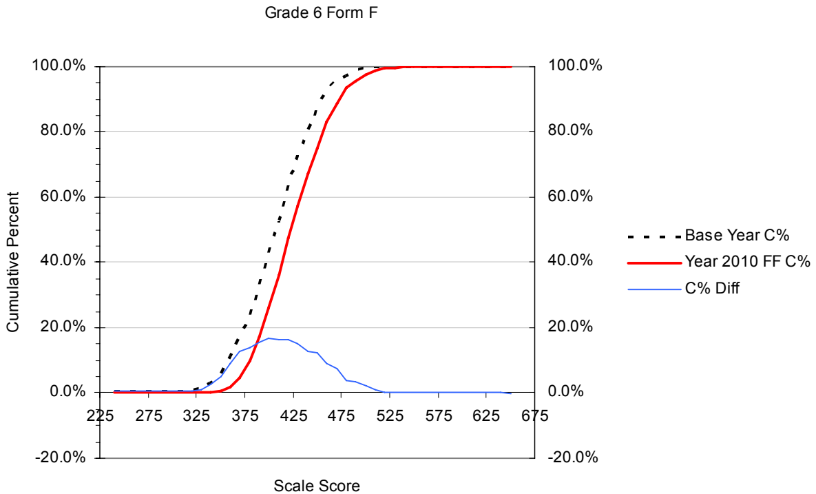
Figure B.28 Cumulative Distribution Functions (CDFs) for the Year 2006 vs. Year 2010 Scale Scores with the Cumulative Percent Differences between CDFs: Grade 6 Form F
