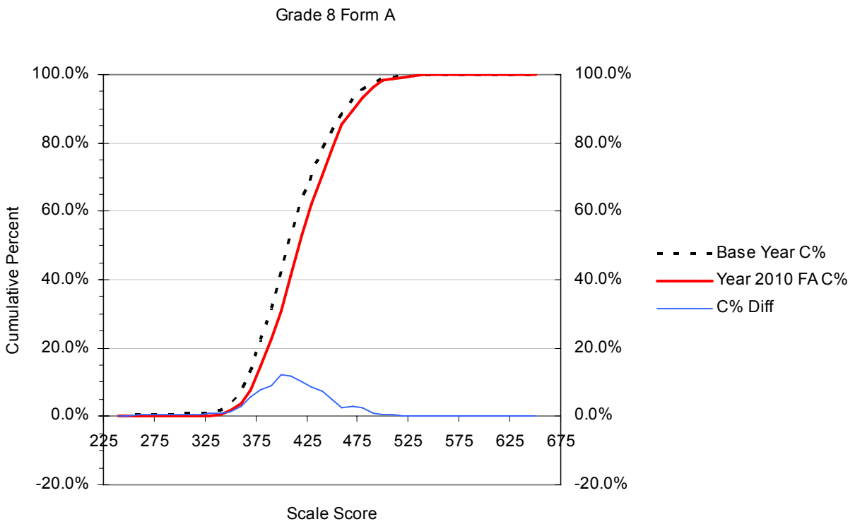
Figure B.39 Cumulative Distribution Functions (CDFs) for the Year 2006 vs. Year 2010 Scale Scores with the Cumulative Percent Differences between CDFs: Grade 8 Form A
