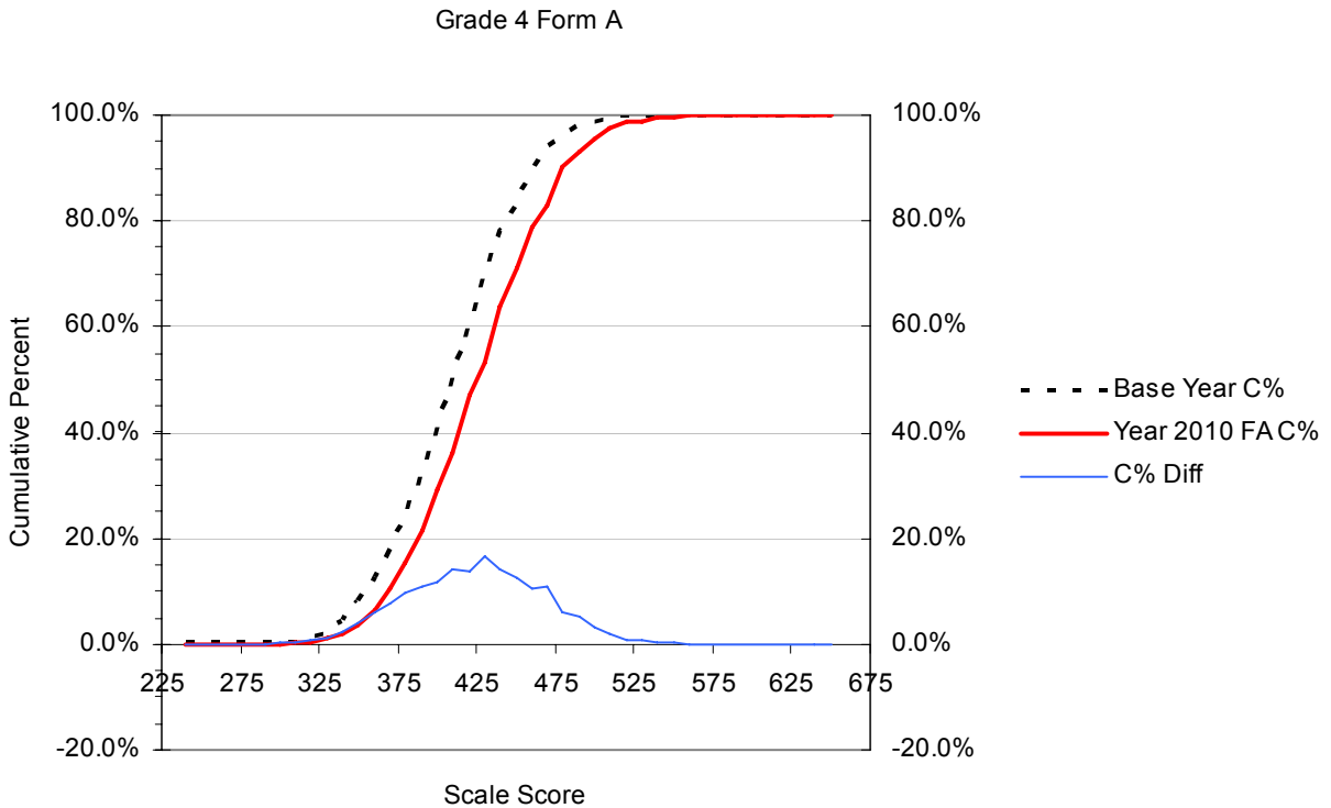
Figure B.11 Cumulative Distribution Functions (CDFs) for the Year 2006 vs. Year 2010 Scale Scores with the Cumulative Percent Differences between CDFs: Grade 4 Form A
