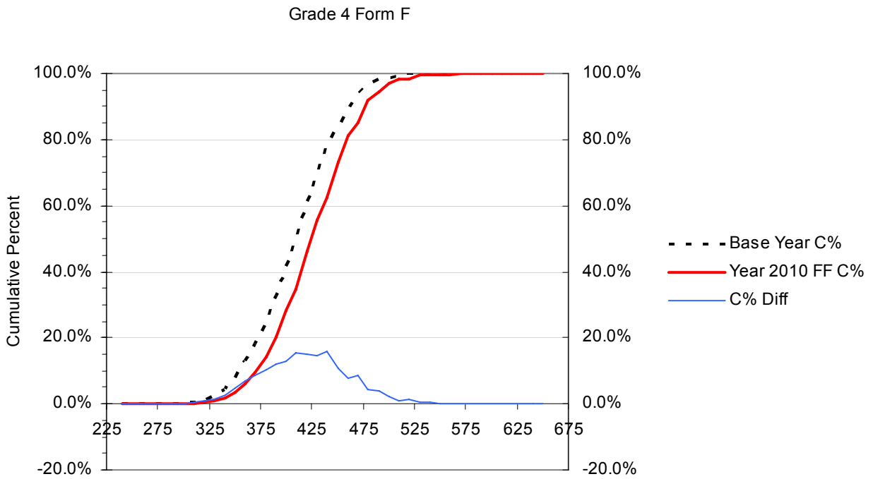
Figure B.14 Cumulative Distribution Functions (CDFs) for the Year 2006 vs. Year 2010 Scale Scores with the Cumulative Percent Differences between CDFs: Grade 4 Form F
