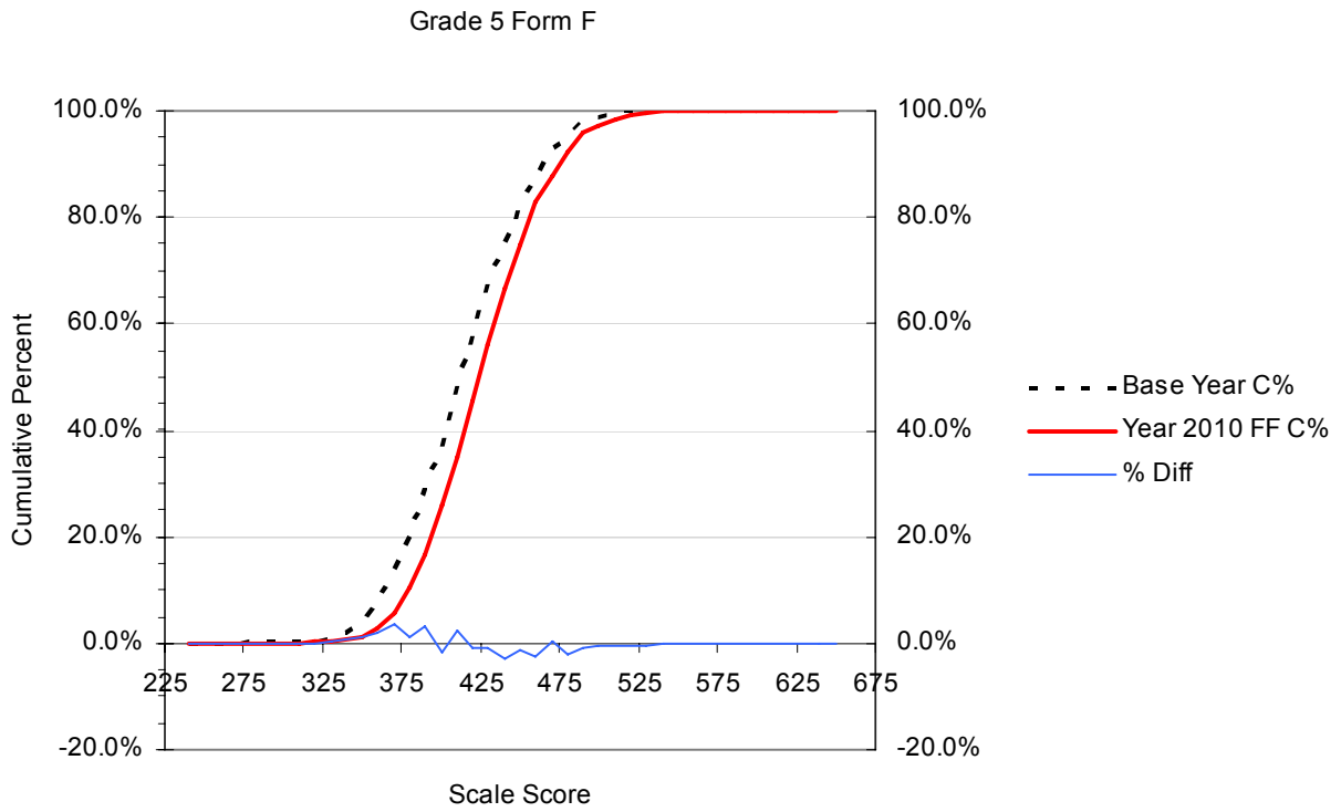
Figure B.20 Cumulative Distribution Functions (CDFs) for the Year 2006 vs. Year 2010 Scale Scores with the Percent Differences between CDFs: Grade 5 Form F
