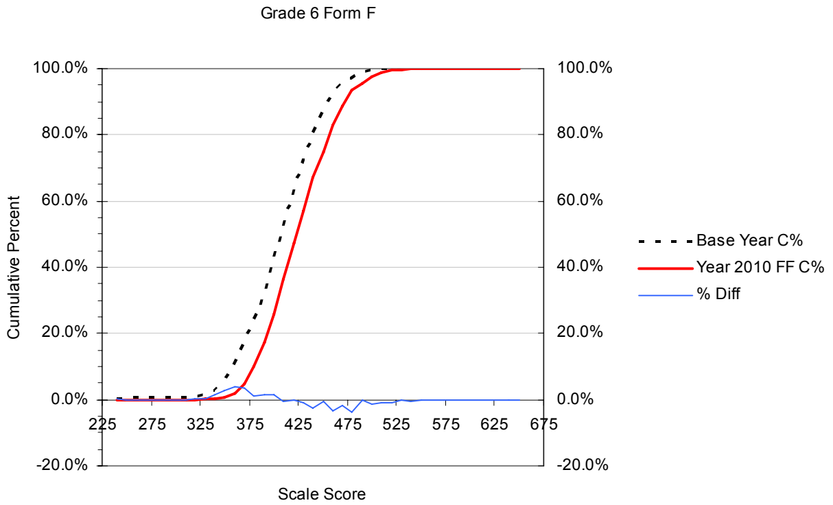
Figure C.27 Cumulative Distribution Functions (CDFs) for the Year 2006 vs. Year 2010 Scale Scores with the Percent Differences between CDFs: Grade 6 Form F
