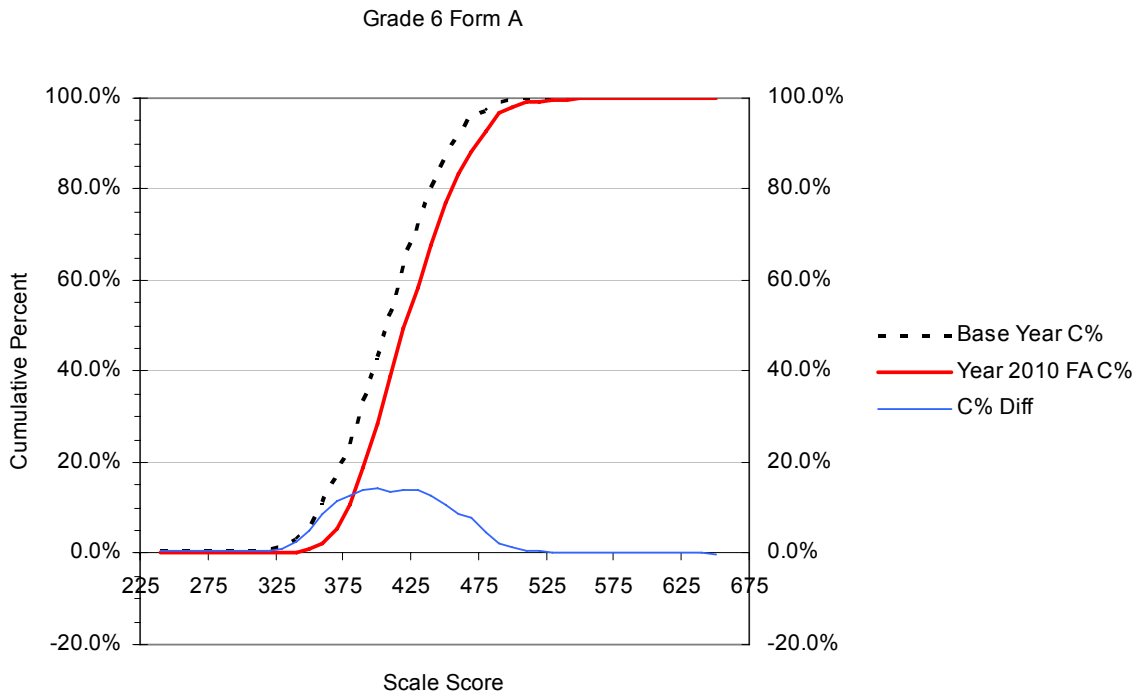
Figure B.25 Cumulative Distribution Functions (CDFs) for the Year 2006 vs. Year 2010 Scale Scores with the Cumulative Percent Differences between CDFs: Grade 6 Form A
