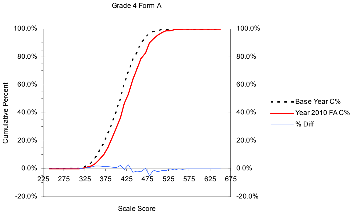
Figure B.10 Cumulative Distribution Functions (CDFs) for the Year 2006 vs. Year 2010 Scale Scores with the Percent Differences between CDFs: Grade 4 Form A
