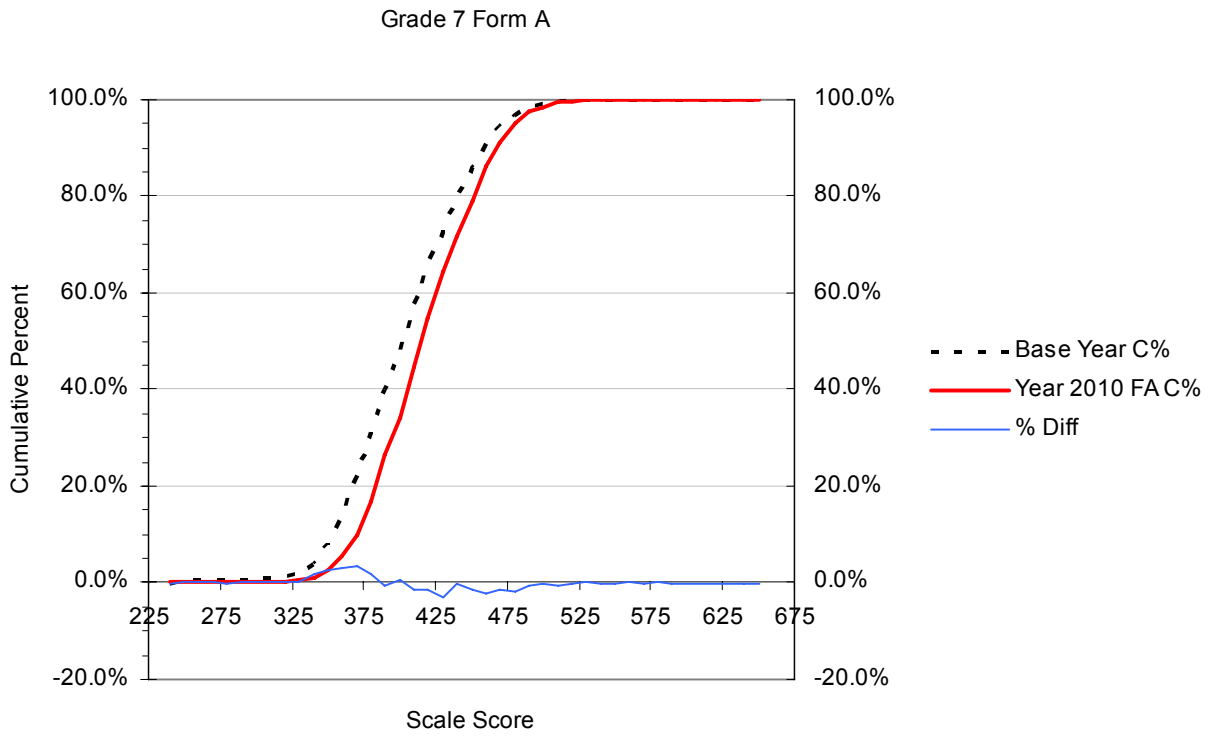
Figure B.31 Cumulative Distribution Functions (CDFs) for the Year 2006 vs. Year 2010 Scale Scores with the Percent Differences between CDFs: Grade 7 Form A
