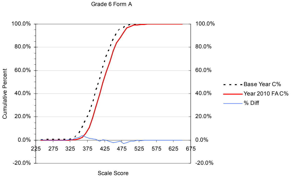
Figure C.24 Cumulative Distribution Functions (CDFs) for the Year 2006 vs. Year 2010 Scale Scores with the Percent Differences between CDFs: Grade 6 Form A
