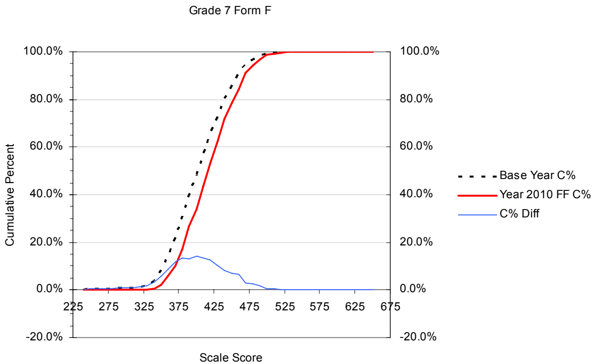
Figure B.35 Cumulative Distribution Functions (CDFs) for the Year 2006 vs. Year 2010 Scale Scores with the Cumulative Percent Differences between CDFs: Grade 7 Form F
