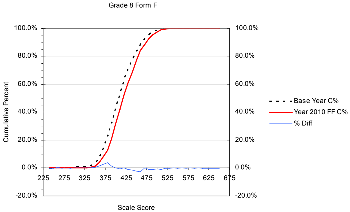
Figure B.41 Cumulative Distribution Functions (CDFs) for the Year 2006 vs. Year 2010 Scale Scores with the Percent Differences between CDFs: Grade 8 Form F
